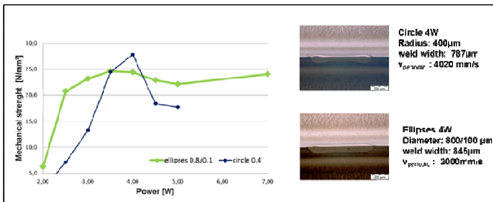
Top: Laser TWIST welding of PP, v=50mm/s, seam width 800µm with TWIST circle and TWIST ellipse.
