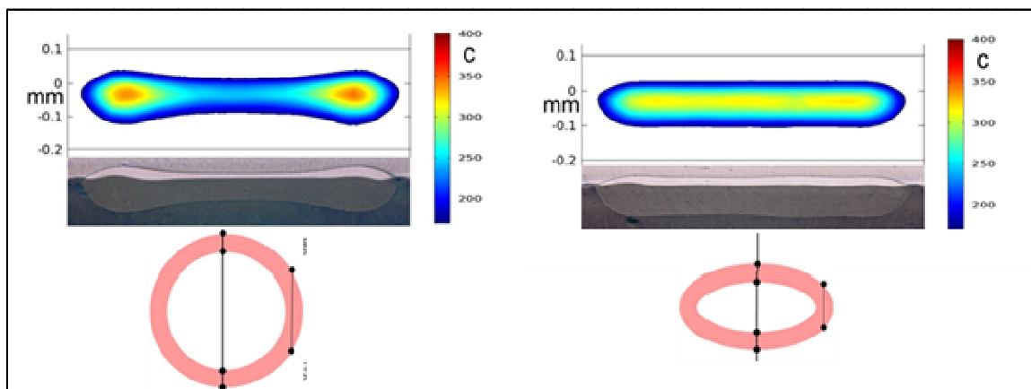
Bottom: Heat affected zones in theory and experiment for Laser TWIST circle and TWIST ellipse welding of PP
